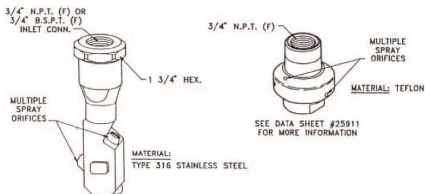
Two types of 360-degree tank rinse nozzles
